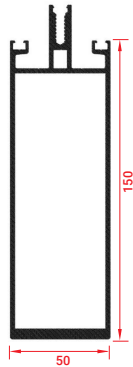
POSTE COLUMNA | POTEAU | COLUMN POST
